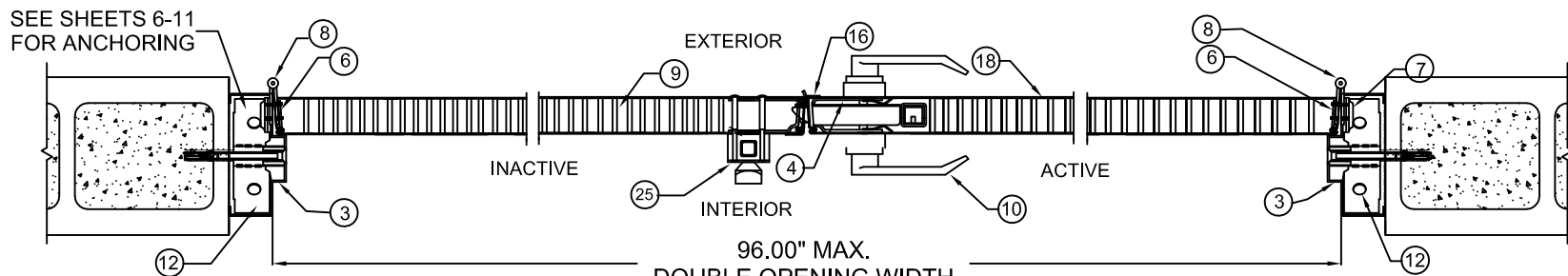
SECTION A-A LM9300 ON ACTIVE LEAF AND 360 SURFACE BOLTS ON INACTIVE LEAF
