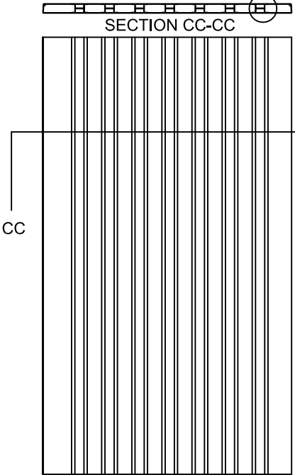
(C) STEEL STIFFENED HAT SHAPED SECTIONS 22 GA. MIN.
