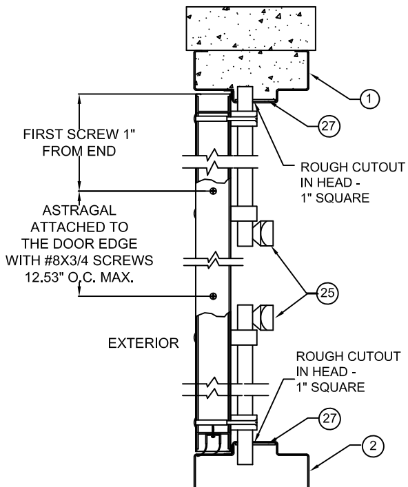
SECTION D-D INACTIVE LEAF WITH IVES 360 SURFACE BOLTS IN TOP AND BOTTOM
