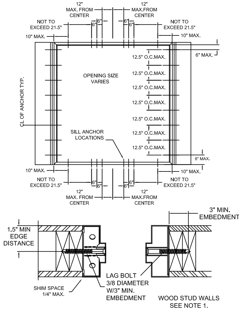
TYPE 1 EMA ANCHORS
