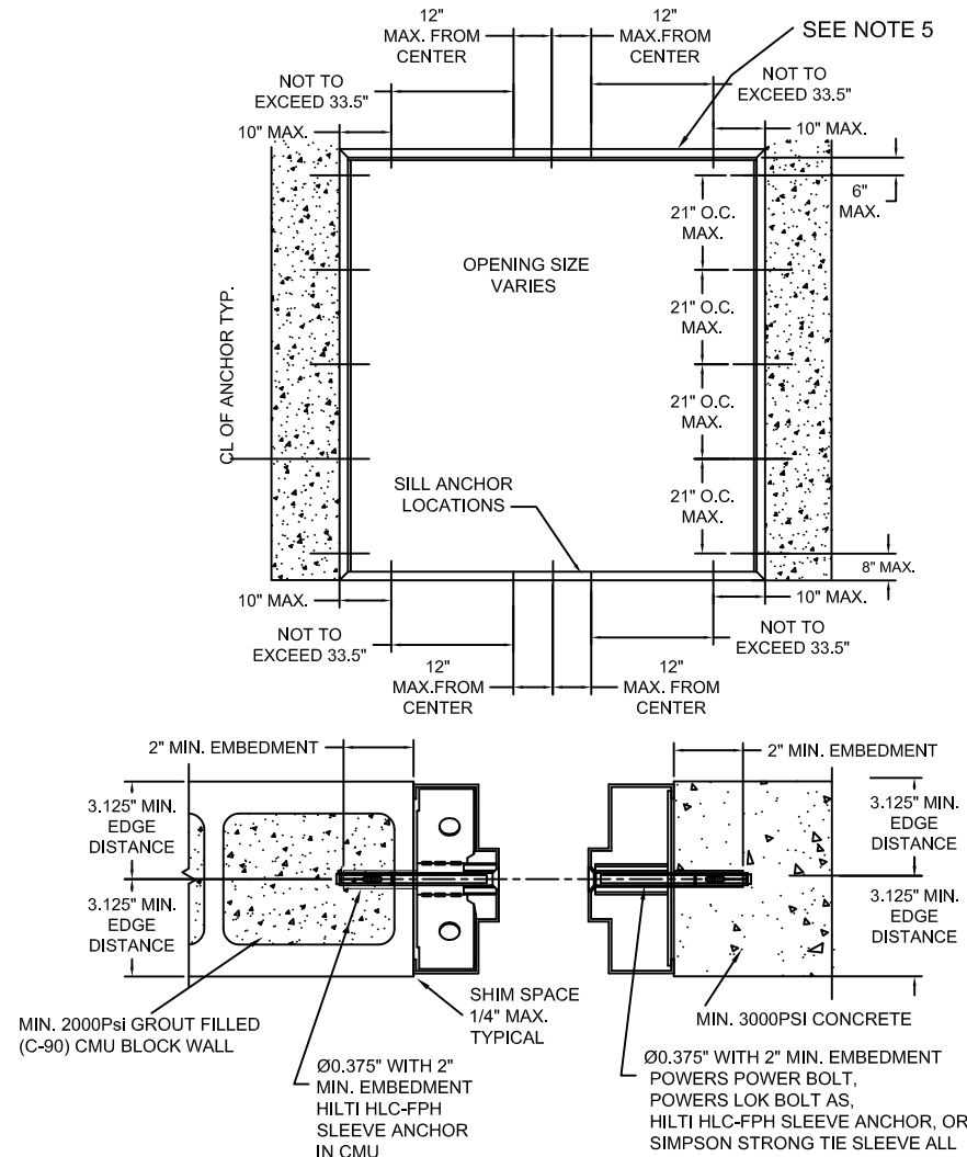
TYPE 1 EMA ANCHORS
