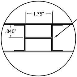
DETAIL 'V1'
