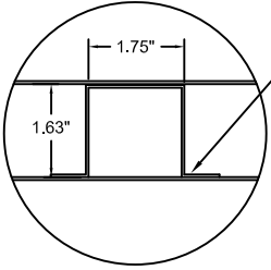
DETAIL 'V2'
