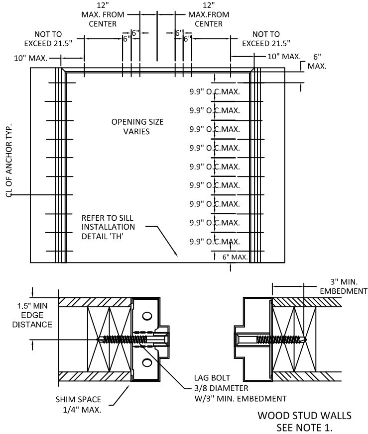
TYPE 1 EMA ANCHORS
