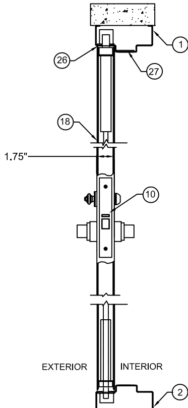
SECTION E-E ACTIVE LEAF WITH THREE POINT DEVICE
