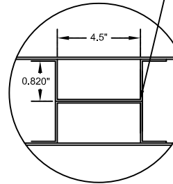
DETAIL 'V3'
