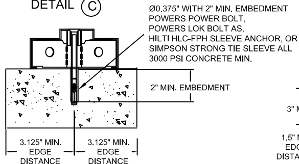
SILL ANCHOR DETAIL (C)
