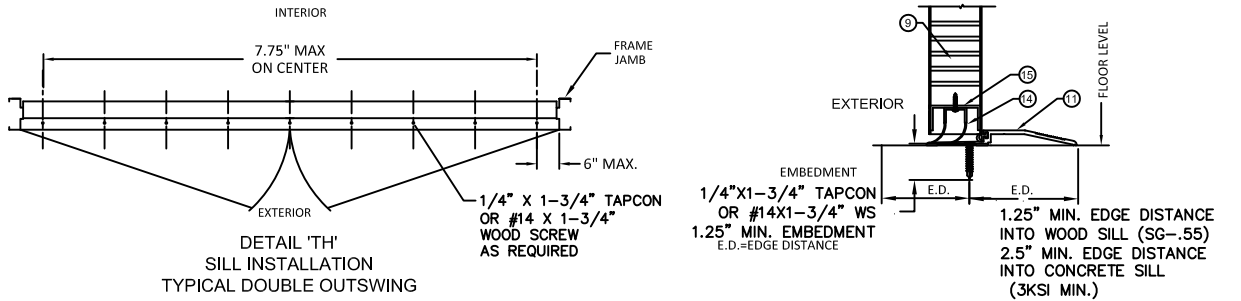
TYPE 1 THRESHOLD DETAIL (SILL) WITH INVERTED BOTTOM RAIL
