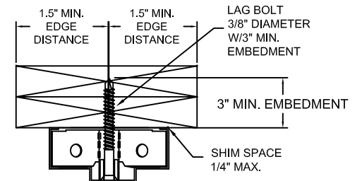
HEAD ANCHOR DETAIL (H2)
