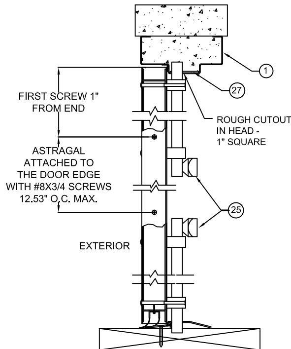
SECTION C-C INACTIVE LEAF WITH IVES 360 SURFACE BOLTS IN TOP AND BOTTOM
