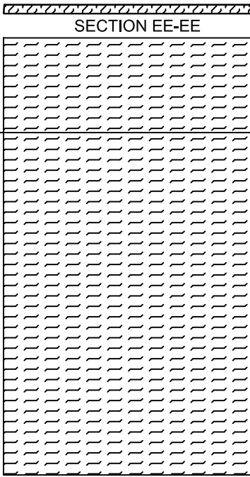
(E) TEMPERATURE RISE CORE MINERAL FIBER BOARD DENSITY: 17 ± 1.5 LBS/FT 3
