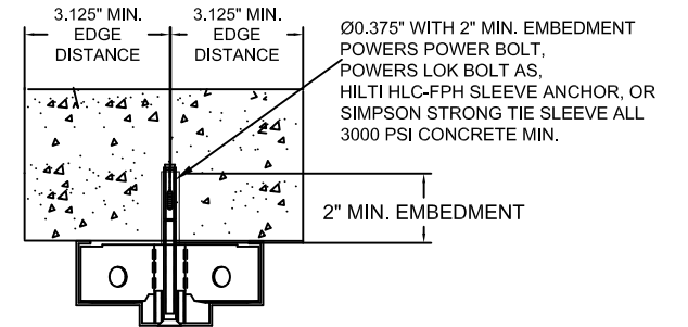
HEAD ANCHOR DETAIL (H1)
