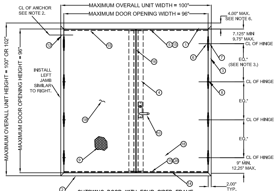
OUTSWING DOOR WITH FOUR SIDED FRAME (EXTERIOR VIEW) ALL DIMENSIONS TYPICAL, UNLESS SPECIFIED OTHERWISE
