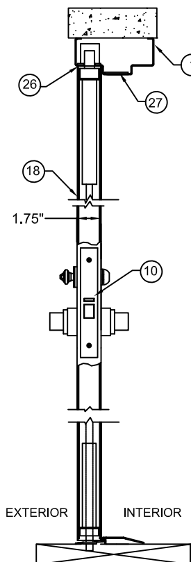
SECTION B-B ACTIVE LEAF WITH THREE POINT DEVICE
